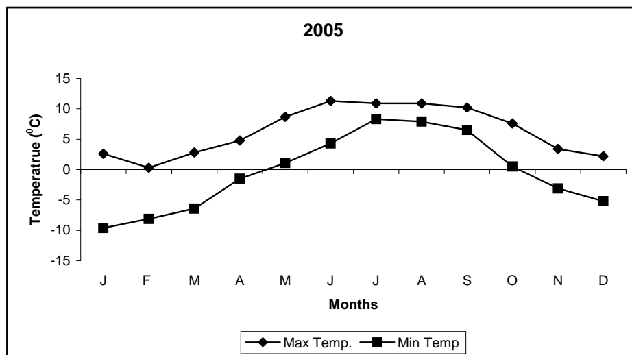
Figure: 1 Monthly Maximum and Minimum temperature (2003-2005) recorded at Kyanjing Gumba, Rasuwa.
